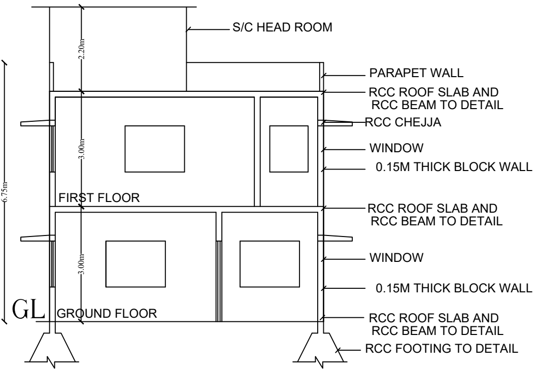
CROSS SECTION AT A-A
